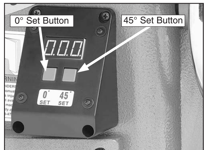
Figure 75. Digital readout.
