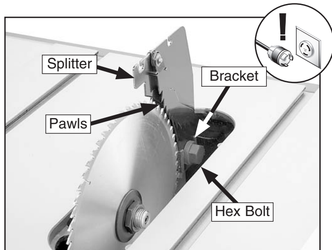
Figure 26. Splitter installed.
