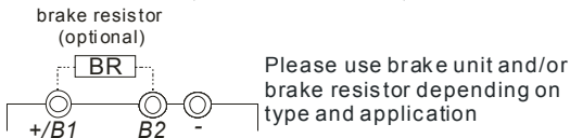
Figure 3 for models of VFD-E Series
