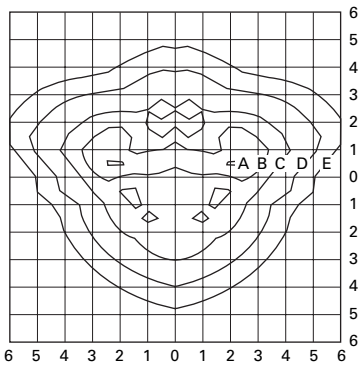
ARC15S31.IES 150-Watt HPS 16,000-Lumen Clear ED-23.5 Lamp Type III Acrylic Refractor
