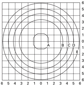
ARC15S51.IES 150-Watt HPS 16,000-Lumen Clear ED-23.5 Lamp Type V Acrylic Refractor
