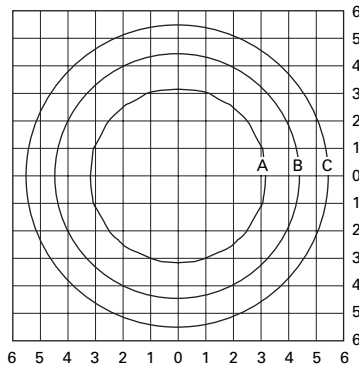
ANG15S55.IES 150-Watt HPS 16,000-Lumen Lamp Type V Glass Refractor
