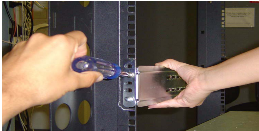
Figure 2-4: Attach Brackets to Post Separate from Shelf Unit
