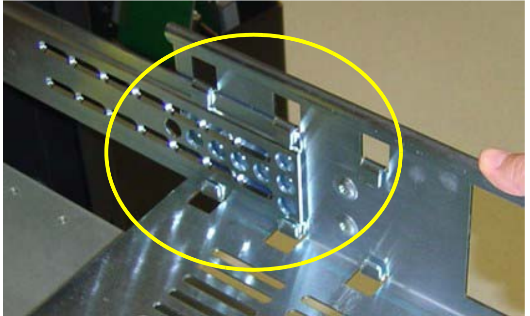
Figure 2-5: Align Shelf with Installed Brackets
