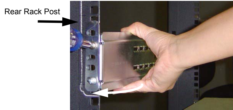
Figure 2-3: Align Bracket with Rear Post
