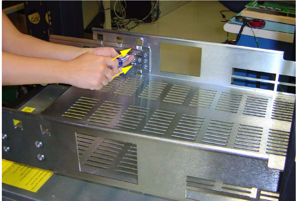
Figure 2-7: Screw the Bracket Into the Shelf From Inside the Rack
