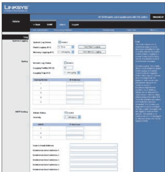
Admin > Log
