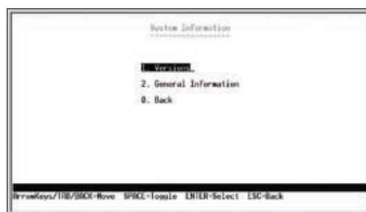
System Information
