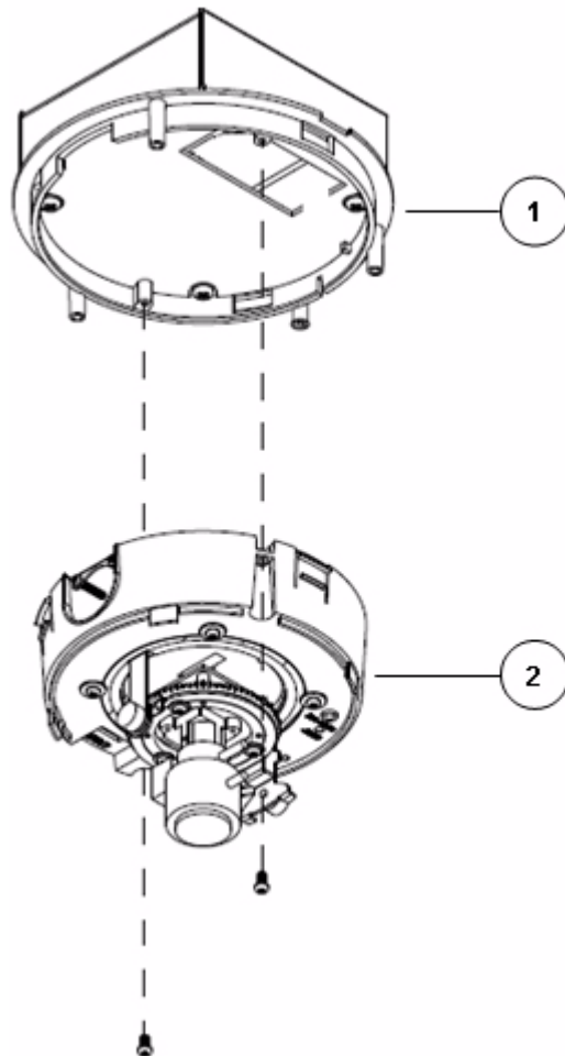
Figure 2-4 Attaching the Camera Unit to the Base Plate
