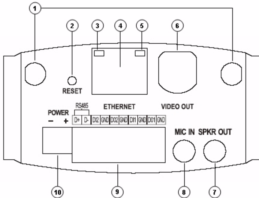
Figure 1-2 Rear of IP Camera
