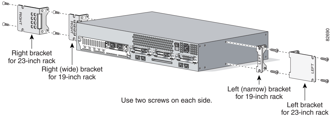
Figure 3 Bracket Installation for Center Mounting with Rear Panel Forward
