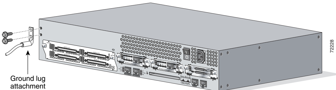
Figure 6 NEBS-Compliant Chassis Ground Connection Using Ground Lug
