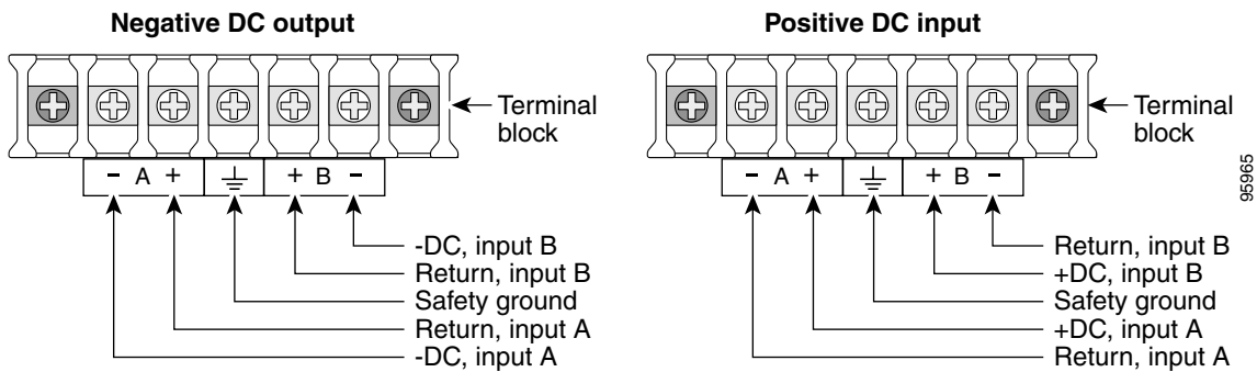
Figure 8 DC Power Connections
