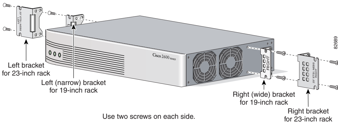
Figure 2 Bracket Installation for Center Mounting with Front Panel Forward
