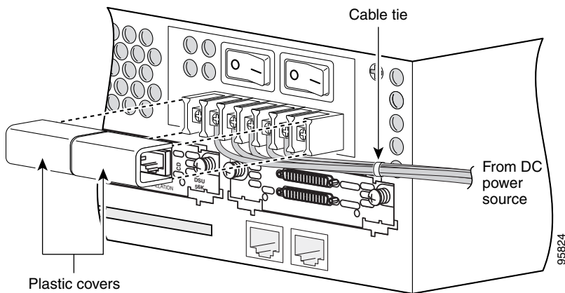
Figure 9 Wire Routing and Attachment
