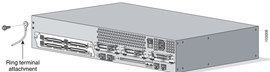
Figure 7 Chassis Ground Connection Using Ring Terminal
