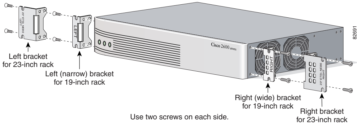
Figure 4 Bracket Installation for Front Mounting
