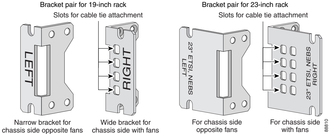
Figure 1 Brackets for Rack-Mounting of Cisco 2691 Routers
