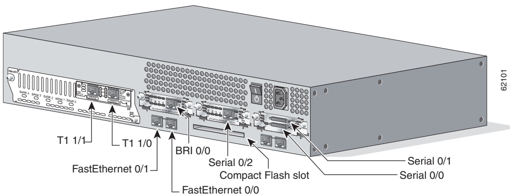
Figure 10 Interface Numbering in Cisco 2691 Routers
