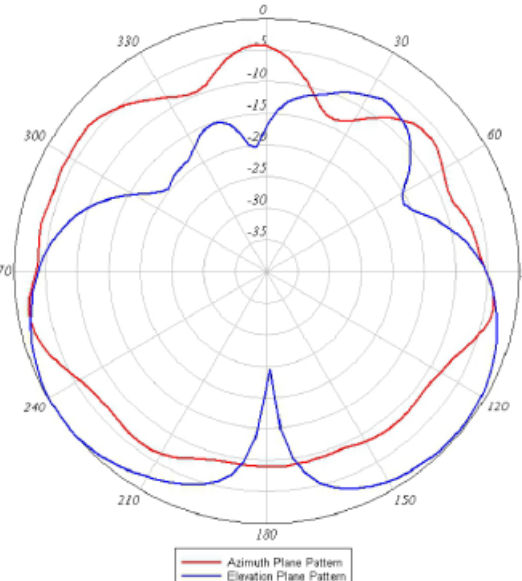
5-GHz Element 4 Azimuth and Elevation Plane Patterns
