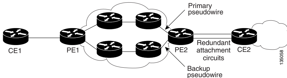
Figure 21-2 Pseudowire Redundancy
