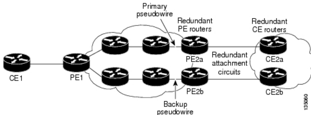
Figure 15-1 Configuring Redundant Pseudowires
