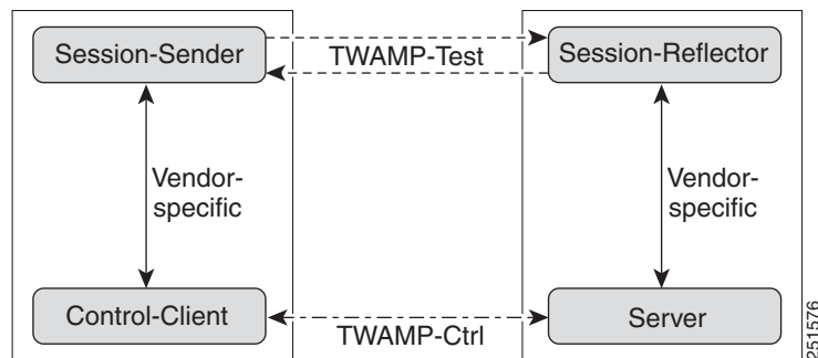
Figure 23-2 TWAMP Architecture
