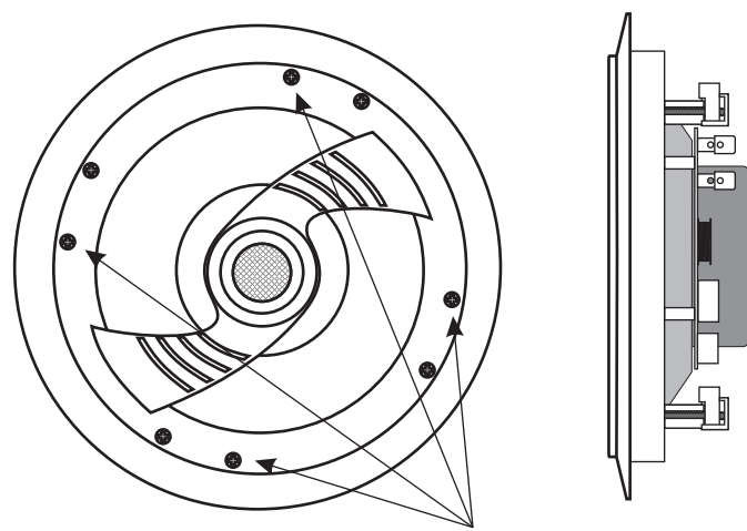
Mounting screws (4)
