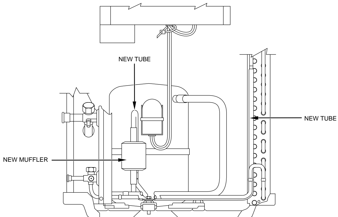
Fig. 1—38TKB024-311 Muffler Kit Installation
