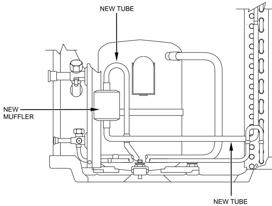
Fig. 1—38TKB024-311 Muffler Kit Installation
