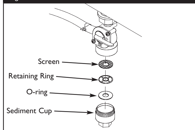
Figure 16 — Fuel Valve Maintenance
