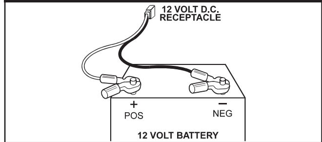
Figure 7 — Battery Connections
