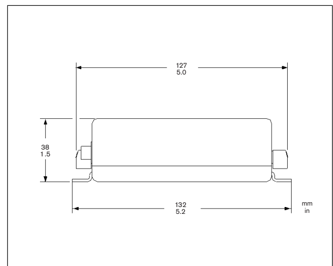
Figure 5 Side Dimensions
