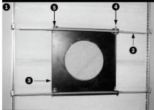
Figure 2.1 Ceiling Mounting (Top View)
