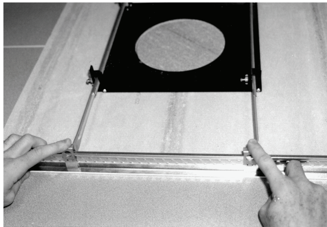
Figure 2.2 Bracket Clip Fitting
