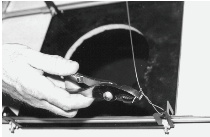
Figure 2.4 Safety Cable Fitment
