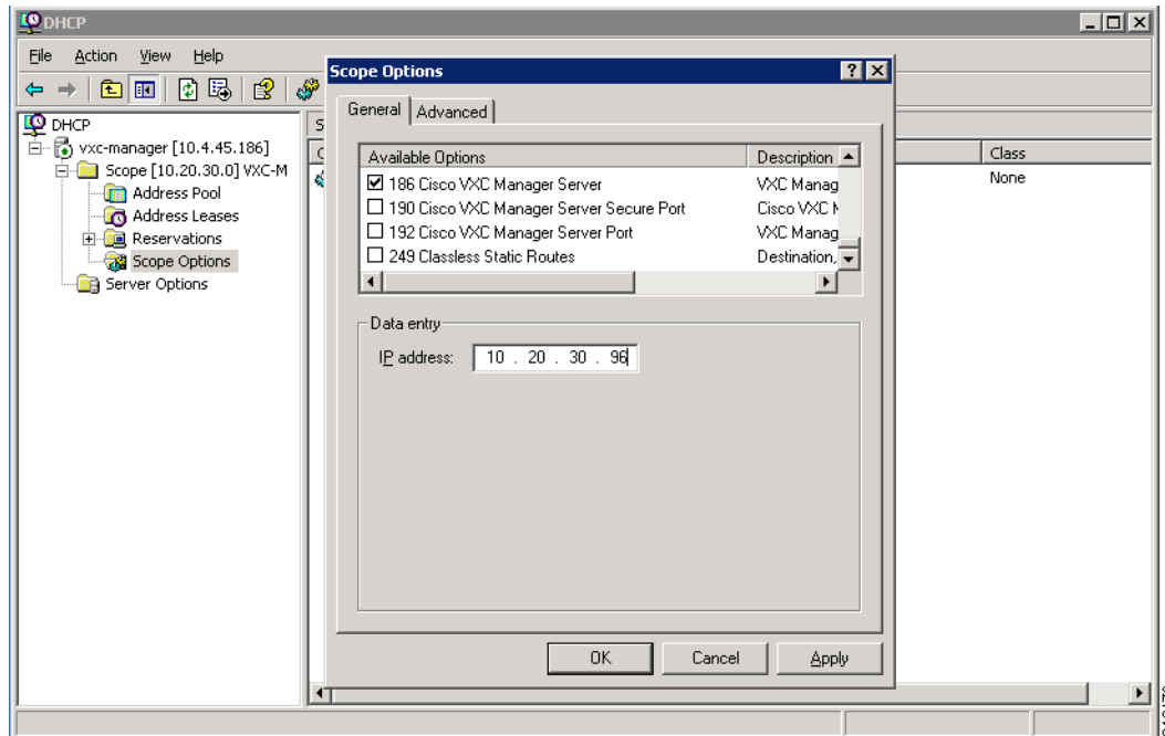
Figure 2-5 DHCP Scope Options: Cisco VXC Manager Server
