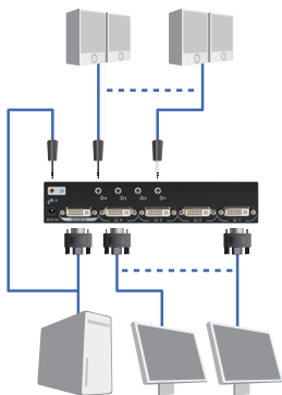
Figure 3-2. AVSP-DVI1X4 connection.
