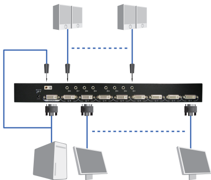
Figure 3-3. AVSP-DVI1X8 connection.
