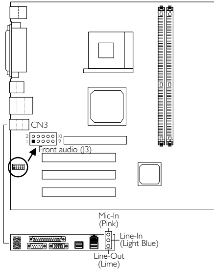
Front Audio (J3)
