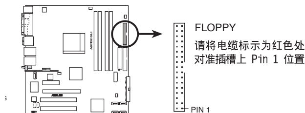
A8N32-SLI Floppy disk drive connector
