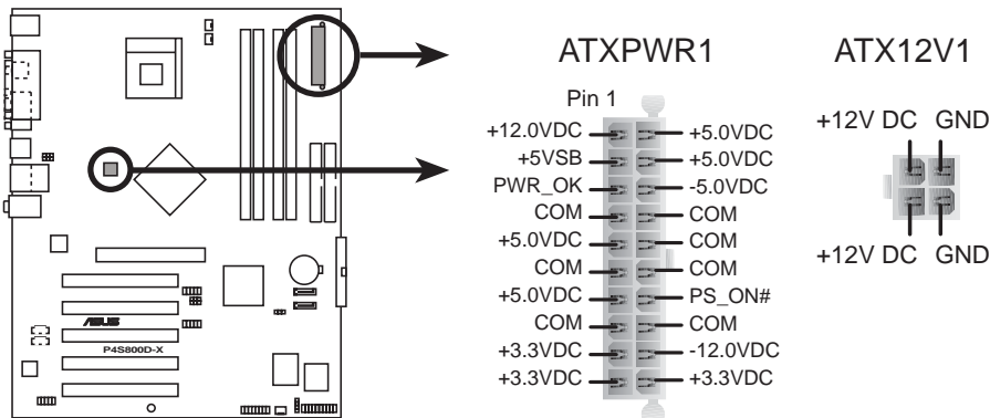
P4S800D-X ATX power connector
