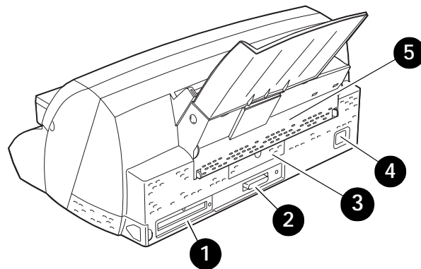
Figure 1.2 Printer Components, Rear View
