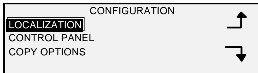
Configuration Screen
