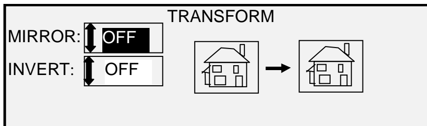
Transform Screen
