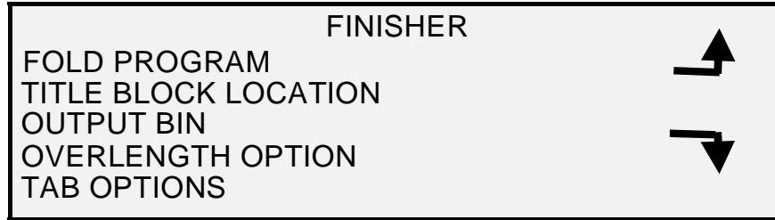
Finisher Screen
