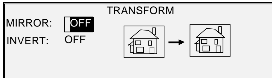
Transform Screen
