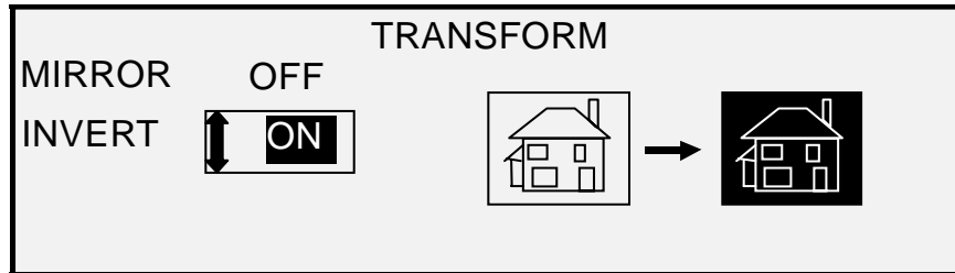
Transform Screen
