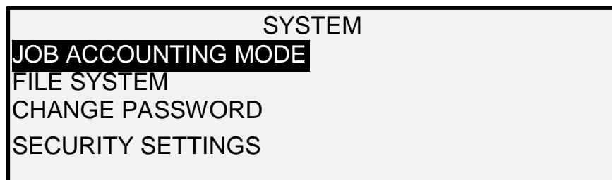
System Screen
