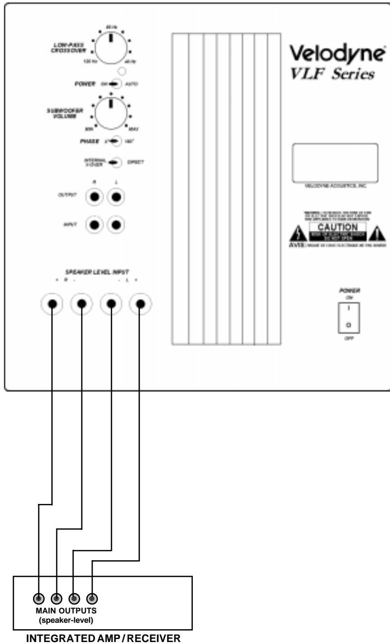
Figure 2. Installation Using Speaker-level (from amplifier) Inputs
