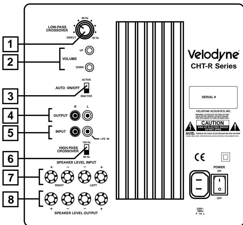
Figure 1. CHT-R Rear Panel Connections
