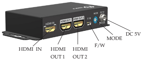
Figure 1: Rear Panel
