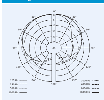
Polar diagram MMD 835-1
