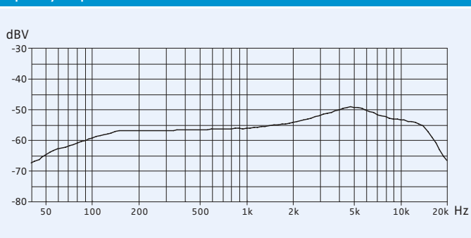
Frequency response curve MMD 845-1
