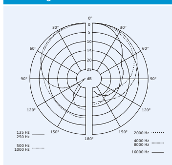
Polar diagram MMD 845-1
