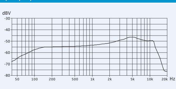
Frequency response curve MMD 835-1
