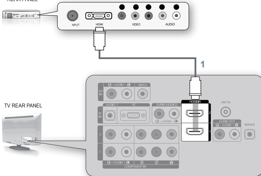
CABLE BOX/SATELLITE RECEIVER (SET-TOP BOX) REAR PANEL
