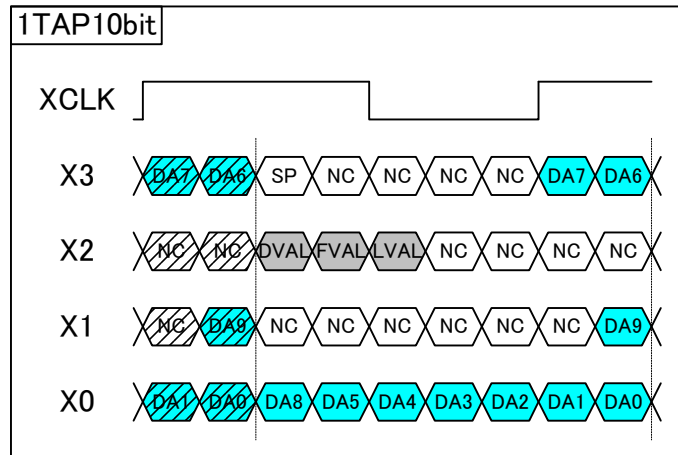
DA0~DA9: 10 bit data for one pixel
