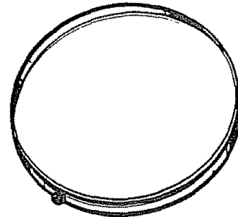
DRAIN PANS AVAILABLE IN 20" DIAMETER FOR WATER HEATERS HAVING A DIAMETER 18" OR LESS AND AVAILABLE IN 26" DIAMETER FOR WATER HEATERS HAVING A DIAMETER 26" OR LESS
