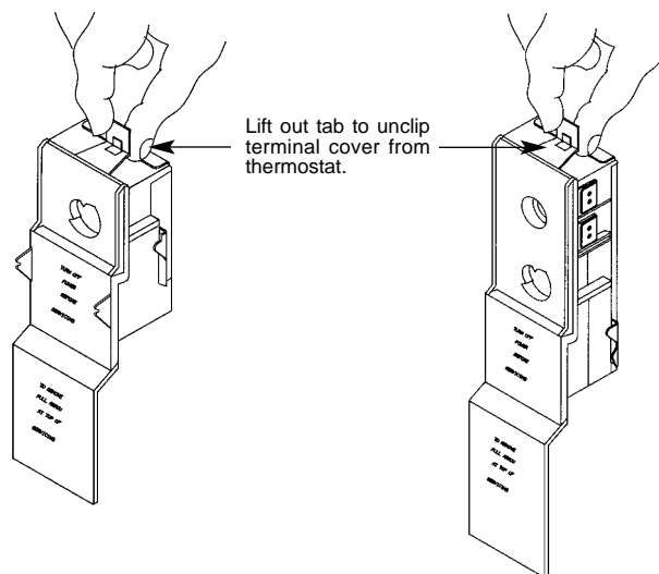
LOWER THERMOSTAT WITHOUT HIGH LIMIT
