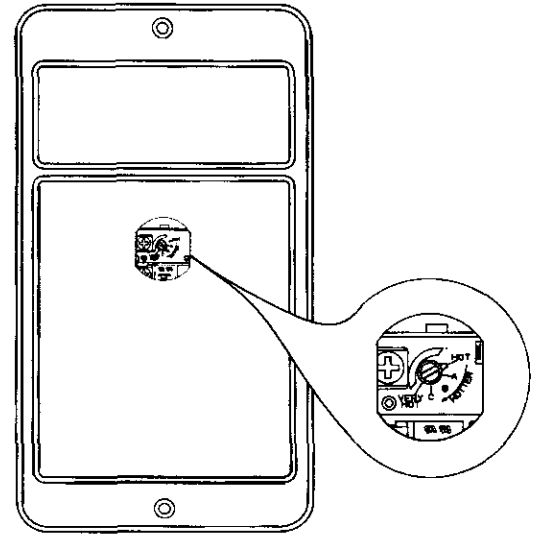
LOWER THERMOSTAT ADJUSTABLE THROUGH OPENING IN LOWER ACCESS PANEL
