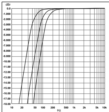
The high pass filter attenuates low frequencies at 12dB per octave. The values given are for the -3dB point.
