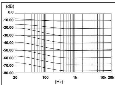
Loudness vs MC-1 Volume control (front left)
