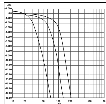
Subwoofer Frequency Response The low pass filter attenuates high frequencies at 24dB per octave. The values given are for the 6dB point.
