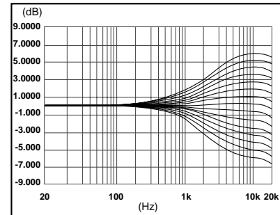
Treble Tone Control Frequency Response
