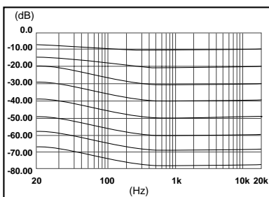
Loudness vs DC-2 Volume control (front left)
