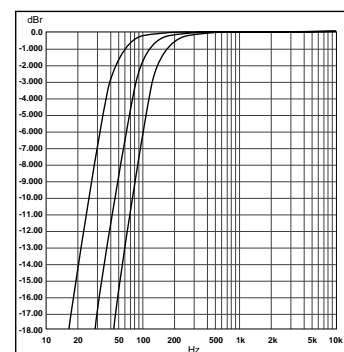
The high pass filter attenuates low frequencies at 12dB per octave. The values given are for the -3dB point.
