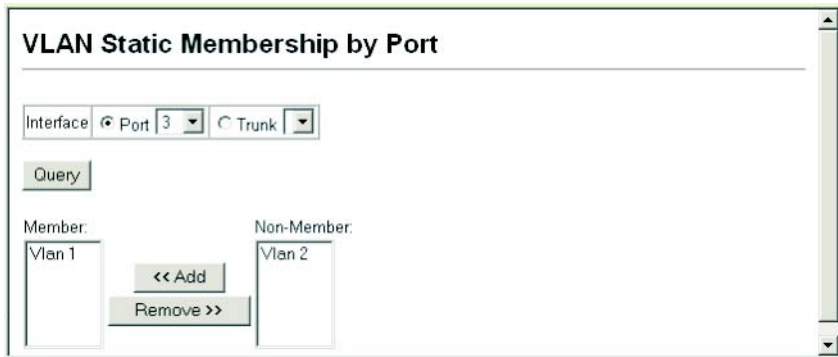
Figure 3-75 VLAN Static Membership
