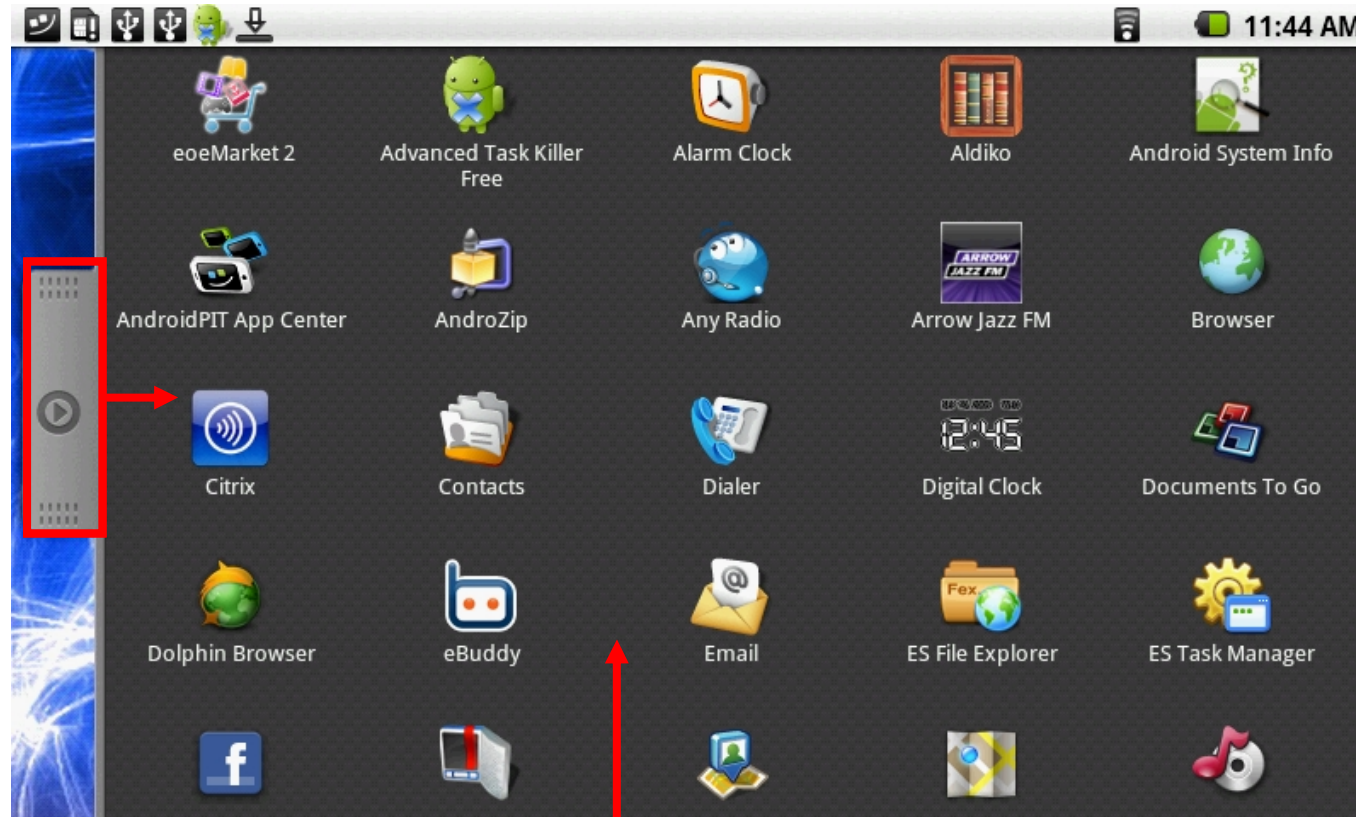
Launcher Screen
