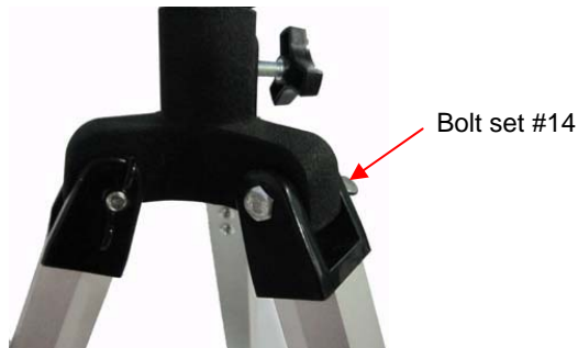
Figure 3. Attach tripod legs to yoke
