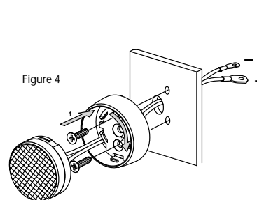
Figure 4 Mounting the tweeter using the I-Mount surface-mounting kit.
