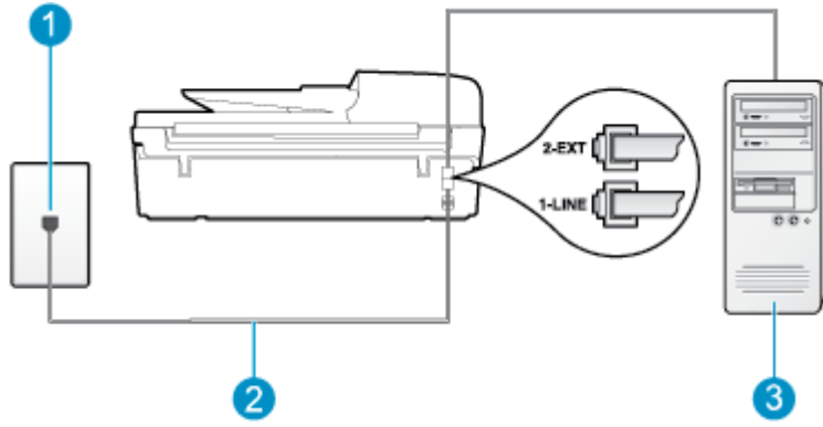
Figure B-6 Back view of the printer
